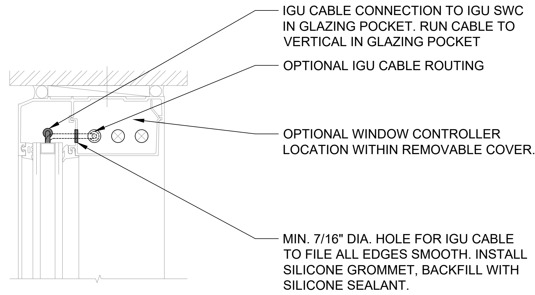
DETAIL 1 HEAD
