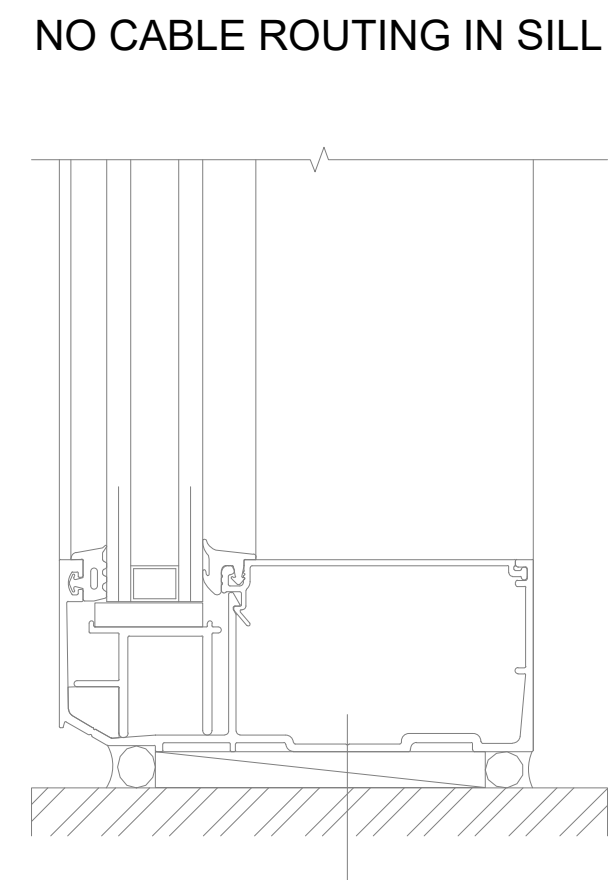
DETAIL 3 SILL
